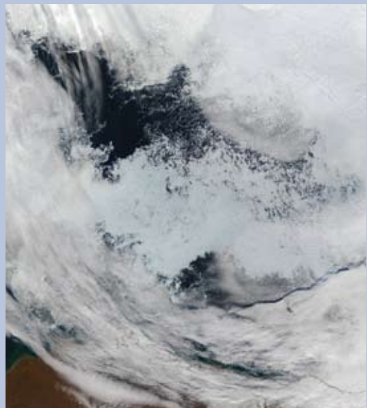
A new polynya formed in the Beaufort Sea in August 2006 and continued to grow. By 11 September 2006, the area of open water had grown to some 100 000 km 2 .
